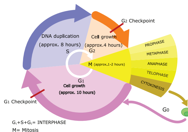
Figure 7.1: Cell cycle
