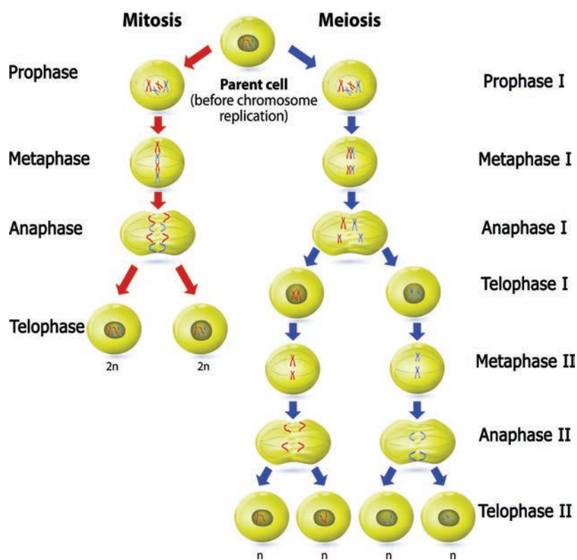
Figure 7.8: Meiosis
