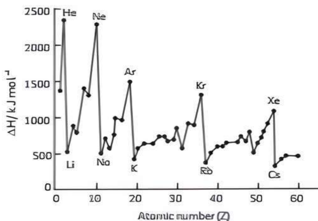
Variation of first ionization enthalpies
