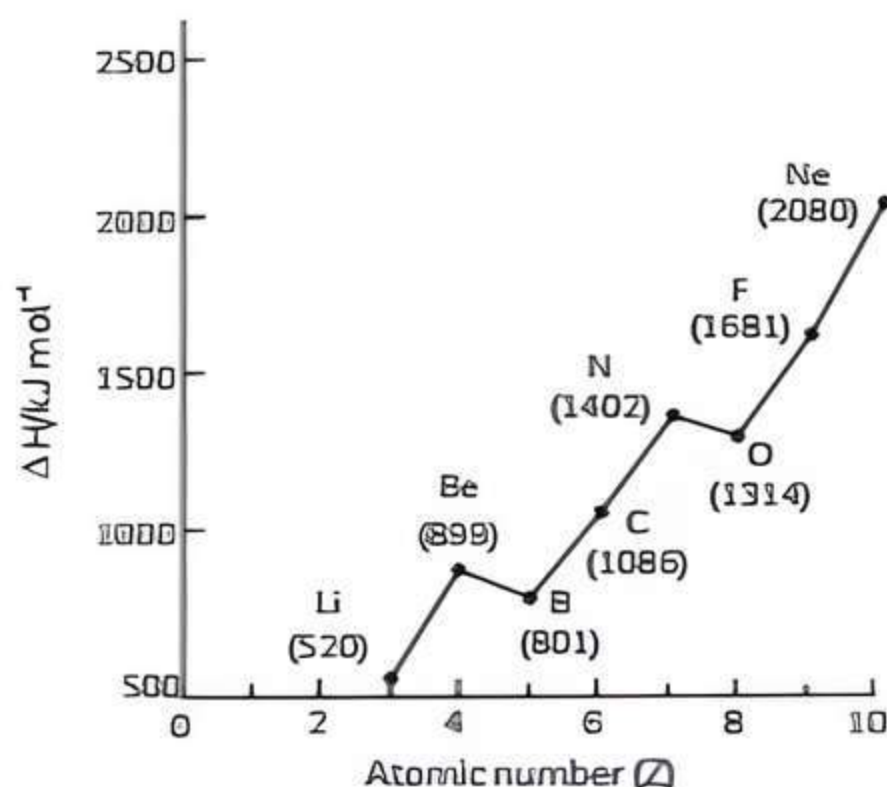
First ionisation enthalpies of elements of the second period as a function of atomic number
