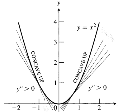
3.28 The graph of f(x) = x^2 on any interval is concave up. □
