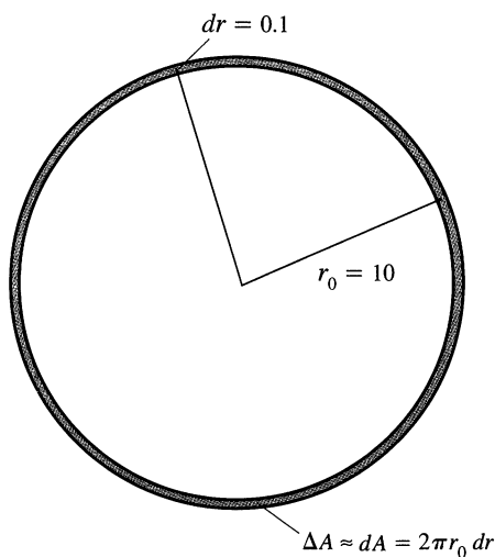
3.66 When dr is small compared with r_0 , as it is when dr = 0.1 and r_0 = 10 , the differential dA = 2\pi r_0 dr gives a good estimate of \Delta A (Example 7).
