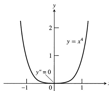
3.32 The graph of y = x^4 has no inflection point at the origin, even though y'' = 0 there.
