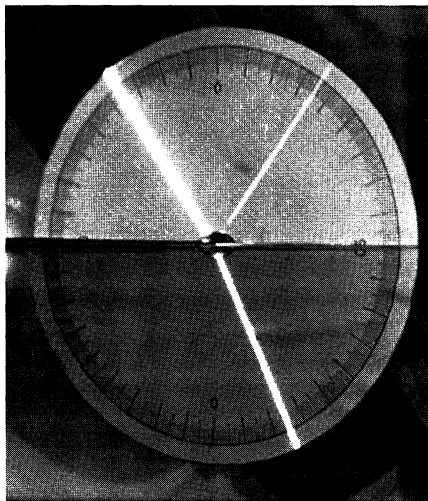
3.56 For air and water at room temperature, the light velocity ratio is 1.33 and Snell's law becomes \sin \theta_1 = 1.33 \sin \theta_2 . In this laboratory photograph, \theta_1 = 35.5^\circ , \theta_2 = 26^\circ , and (\sin 35.5^\circ / \sin 26^\circ) \approx 0.581 / 0.438 \approx 1.33 , as predicted.
