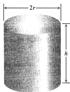
3.50 This 1-L can uses the least material when h = 2r (Example 2).
