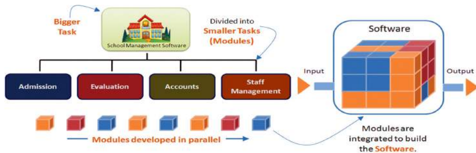
Fig. 31: Modular programming style
