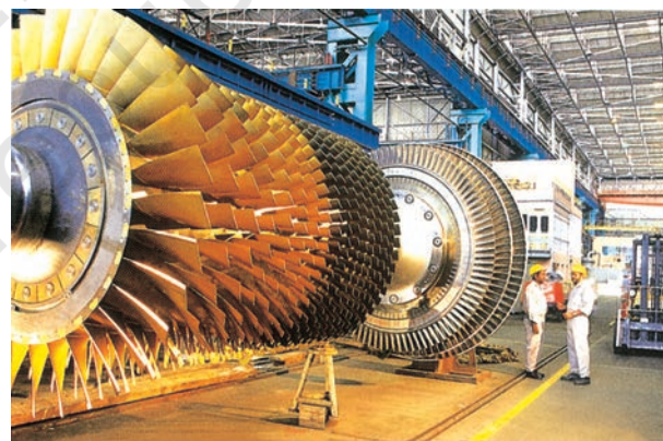
Fig. 6.10: Gas turbine rotor an assembly bed at BHEL, Hyderabad
