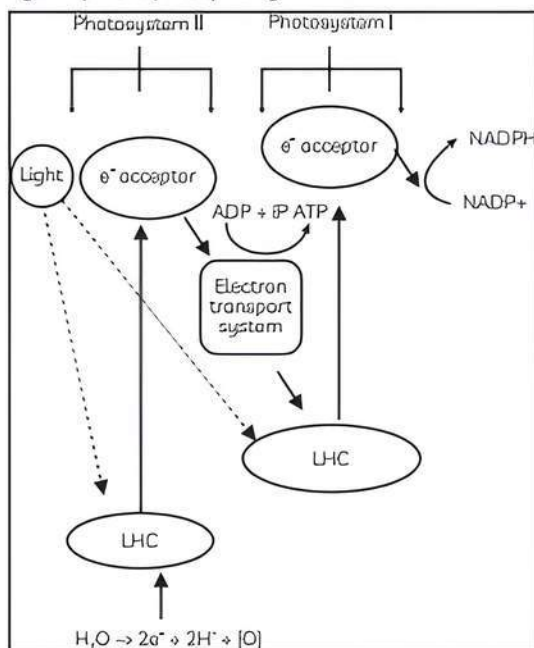
Diagrammatic representation of non-cyclic photophosphorylation
