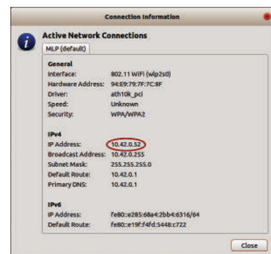
Fig. 5.6 Connection Information Window
