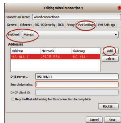
Fig. 5.7 Edit Connection Window
