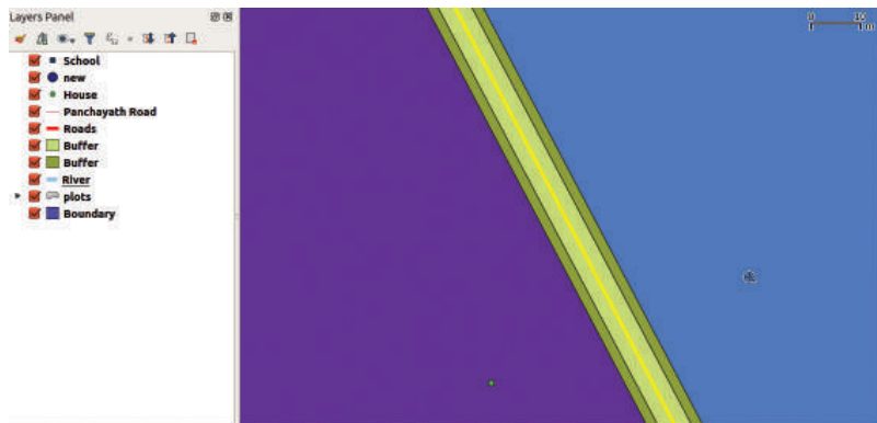
Fig. 6.12 Buffer road
