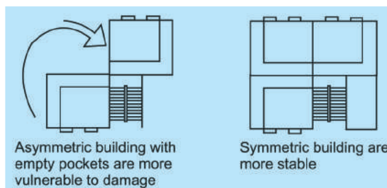
Fig. 2 Desirable orientation & plan form for reducing wind damage.
