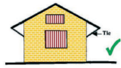
Fig. 5 RIGHT: Avoid large overhangs and use ties
