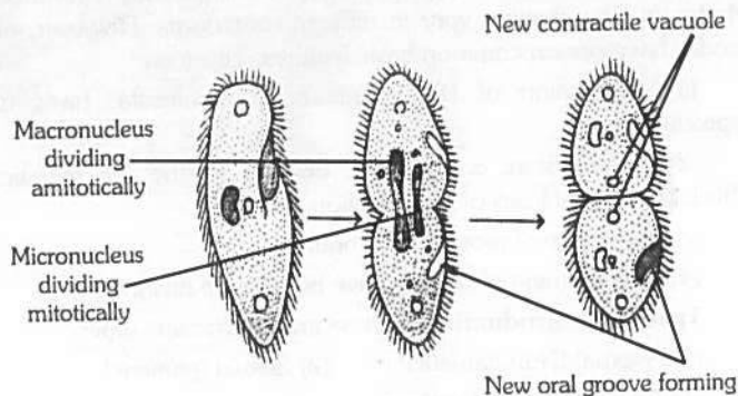
Fig : 6.1-2 Transverse binary fission in paramecium
