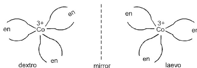
d and \ell of [Co(en)_3]^{3+}
