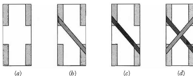
Figure 21 Preparation of an \text{Al}/\text{Al}_2\text{O}_3/\text{Sn} sandwich. (a) Glass slide with indium contacts. (b) An aluminum strip 1 mm wide and 1000 to 3000 Å thick has been deposited across the contacts. (c) The aluminum strip has been oxidized to form an \text{Al}_2\text{O}_3 layer 10 to 20 Å in thickness. (d) A tin film has been deposited across the aluminum film, forming an \text{Al}/\text{Al}_2\text{O}_3/\text{Sn} sandwich. The external leads are connected to the indium contacts; two contacts are used for the current measurement and two for the voltage measurement. (After Giaever and Megerle.)
