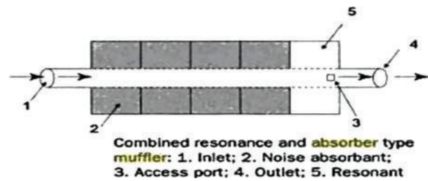
Figure 6.12.3(e) Combined Resonance and Absorber Type
