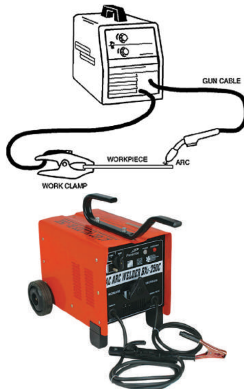
Figure 2.2.3 Welding Machine
