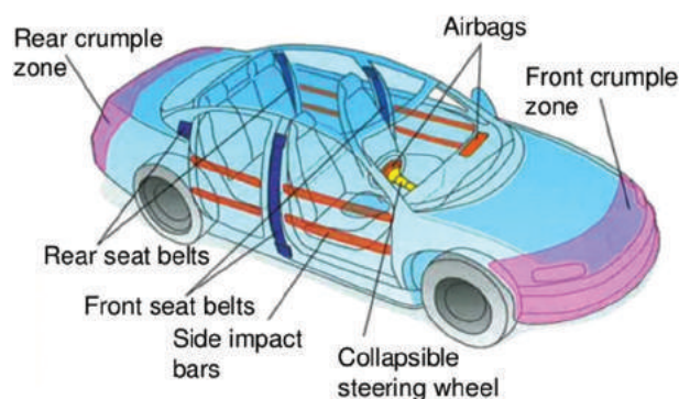
Figure 1.6 Vehicle Safety
