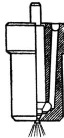
Figure 6.10.3(a) Pintle Nozzle
