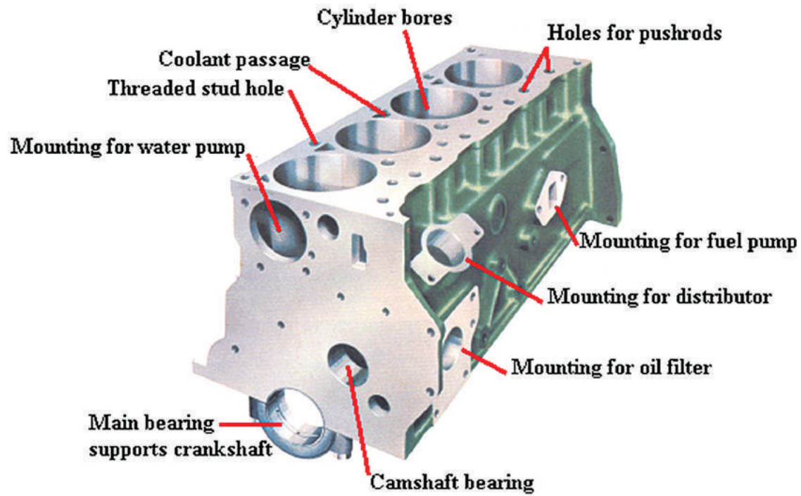
Mono Block
