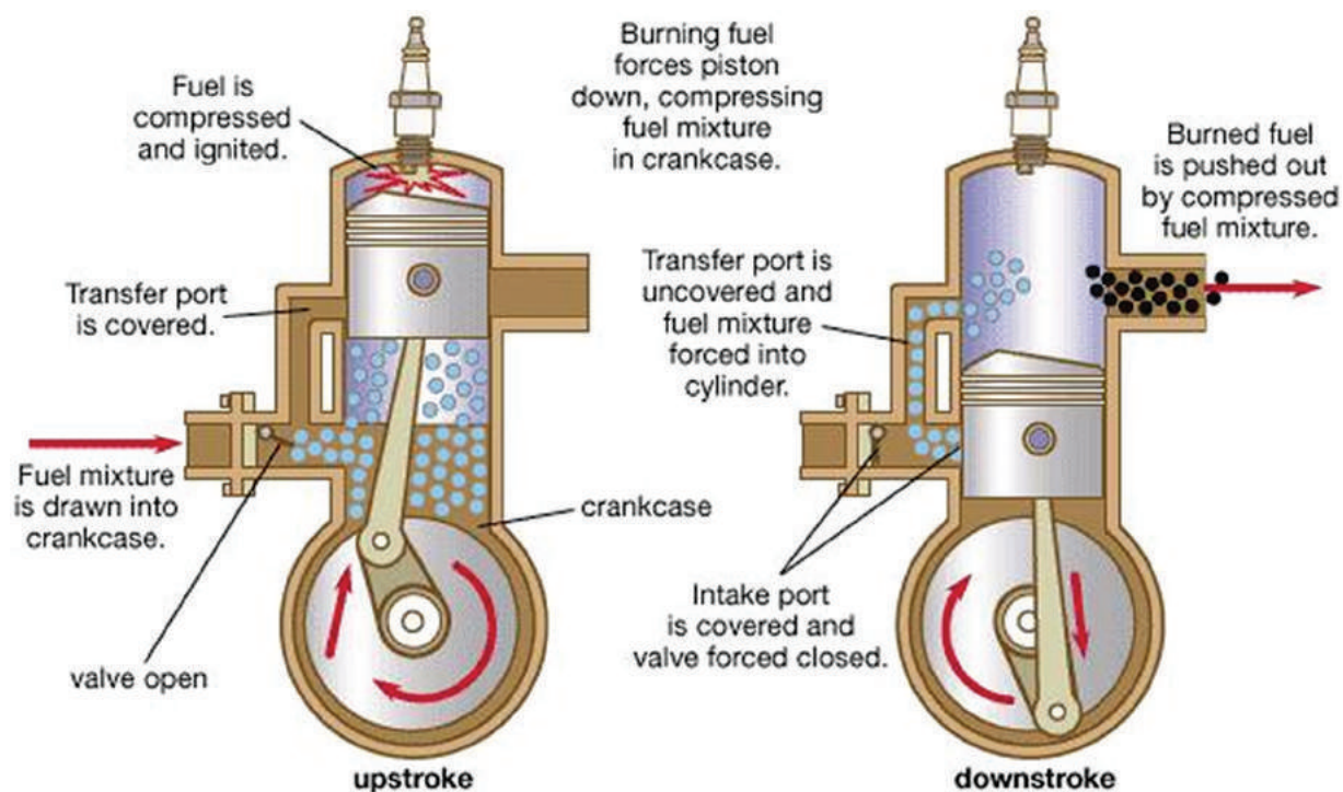
Figure 5.5(b) Upward and Downward Stroke of Two Stroke Petrol Engine
