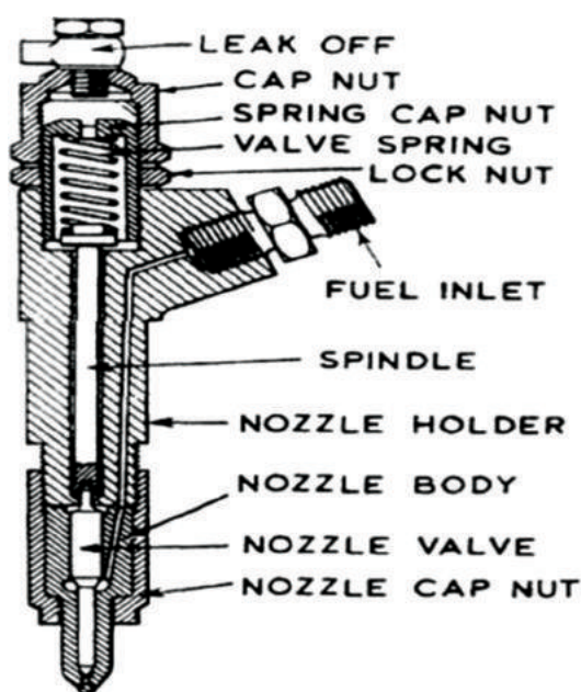
Figure 6.9 Fuel Injector
