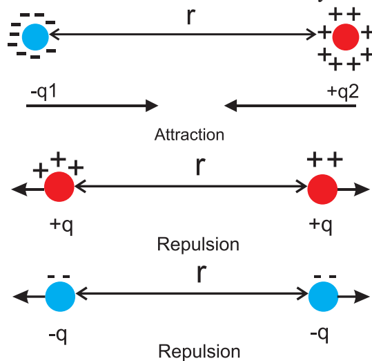
Fig. 10.3: Coulomb's law.
