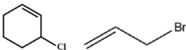
Allylic halide
