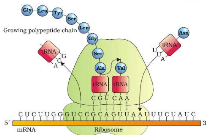
Figure 6.13 Translation
