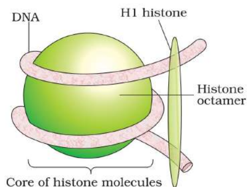
Figure 6.4a Nucleosome
