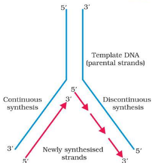
Figure 6.8 Replicating Fork
