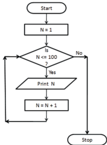
Fig. 3.13 : Flowchart to print numbers from 1 to 100
