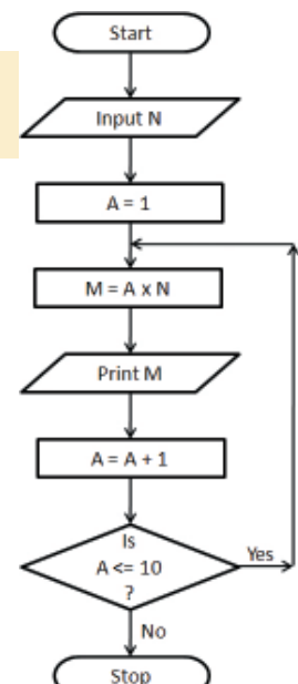
Fig. 3.17 : Flowchart for the first 10 multiples of a number
