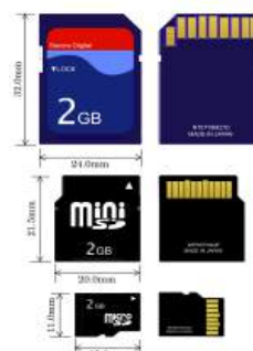
Fig. 2.20 : Flash memory cards
