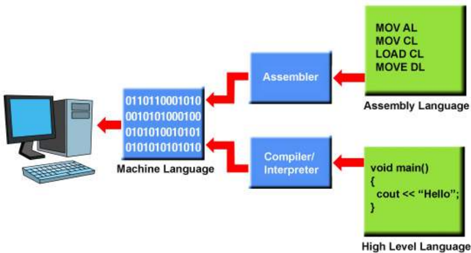
Fig. 2.56: Language processing
