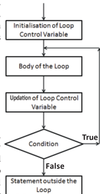
Fig. 7.5 : Flowchart of do...while loop
