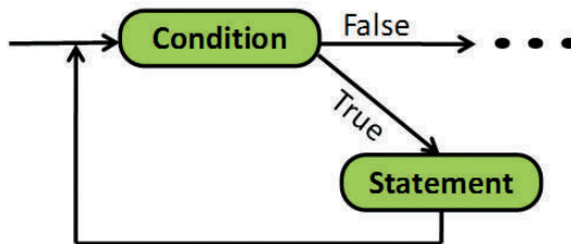
Fig. 3.14 : Looping construct
