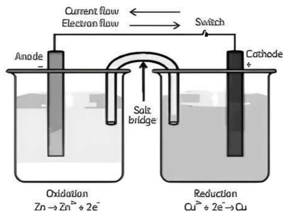
Galvanic Cell
