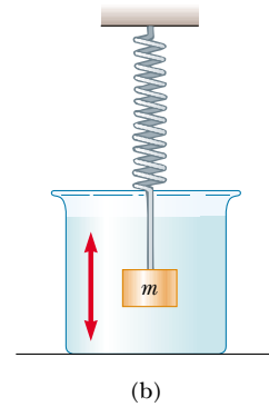
Figure 13.19 (a) Graph of displacement versus time for a damped oscillator. Note the decrease in amplitude with time. (b) One example of a damped oscillator is a mass attached to a spring and submersed in a viscous liquid.
