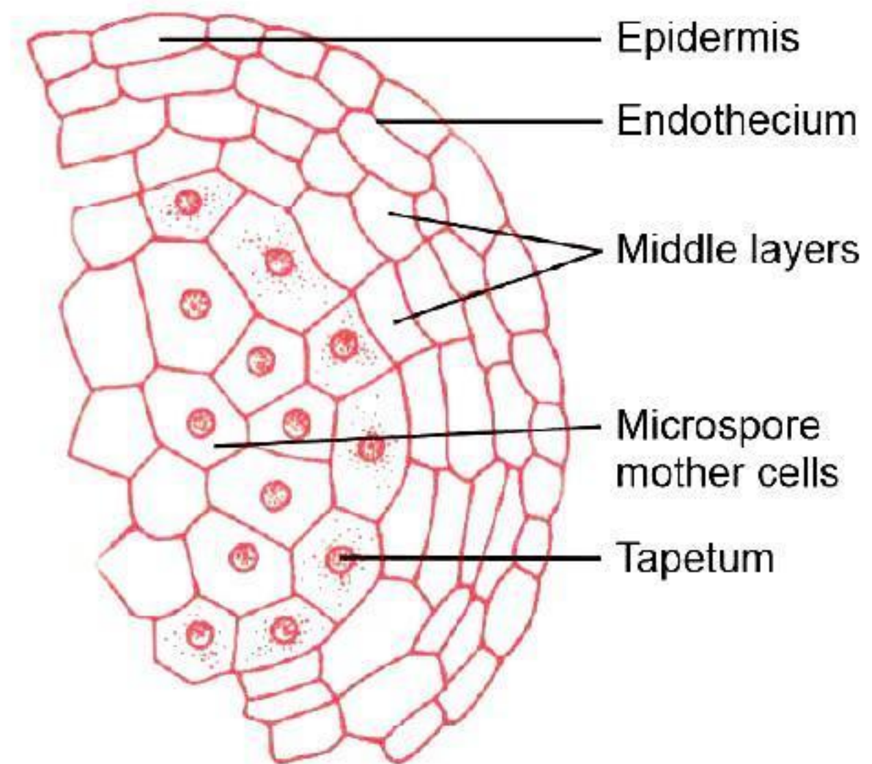
Enlarged view of one microsporangium showing wall layers
