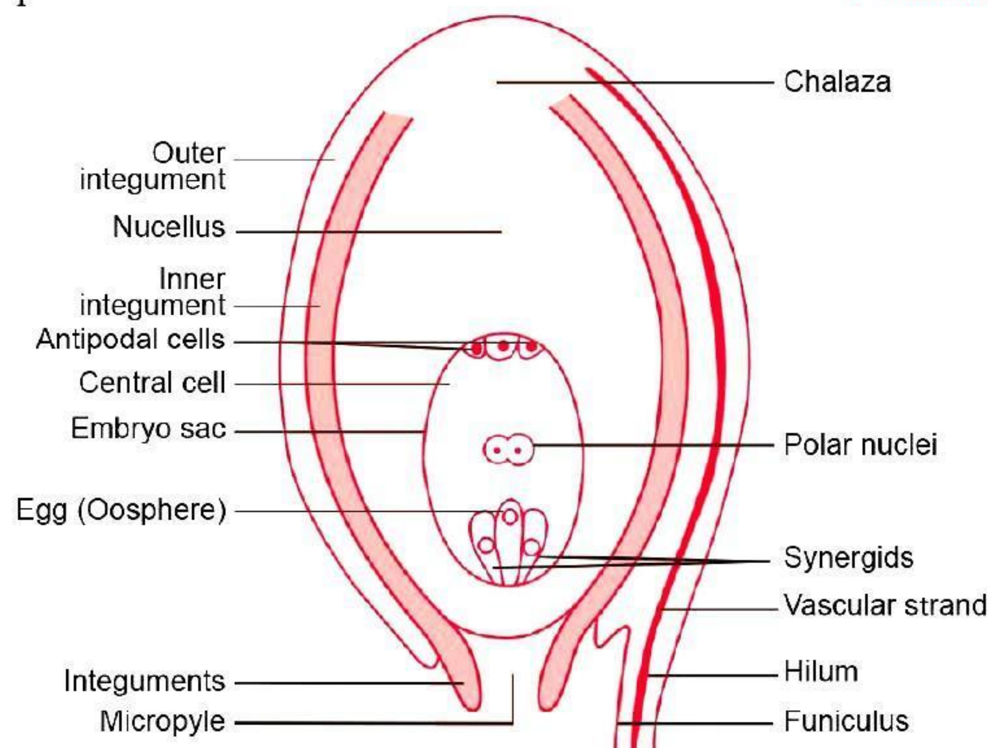
A diagrammatic view of a typical anatropous ovule
