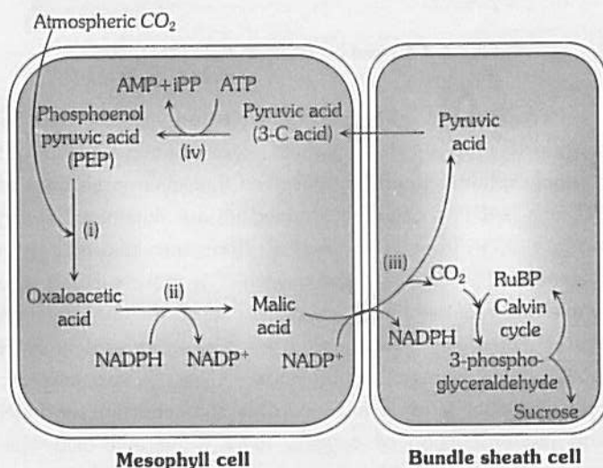
Fig : 4.3-8 Hatch-slack's pathway (cycle) Enzyme : (i) Phosphoenol pyruvate carboxylase, (ii) Malate dehydrogenase, (iii) Decarboxylase, (iv) Pyruvate orthophosphate dikinase
