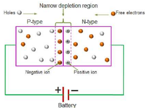
Forward bias
