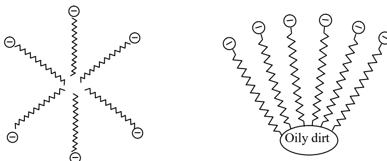
(c) Micelle Formed by detergent molecules in water The hydrocarbon tails stick the oily dirt
