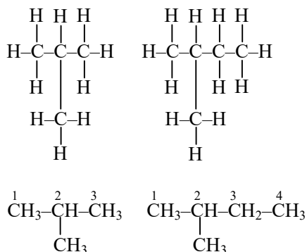
2-Methylpropane 2-Methylbutane
