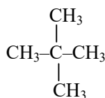
2,2-Dimethylpropane
