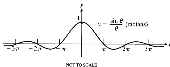
2.33 The graph of f(\theta) = (\sin \theta)/\theta .
