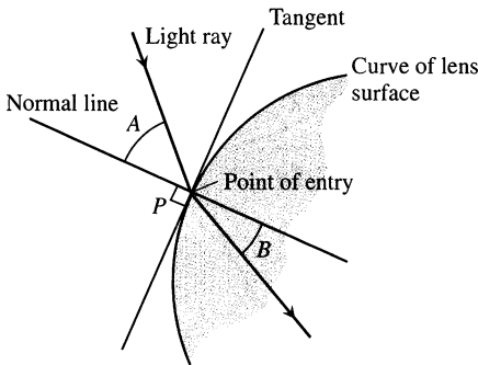
2.48 The profile of a lens, showing the bending (refraction) of a ray of light as it passes through the lens surface.
