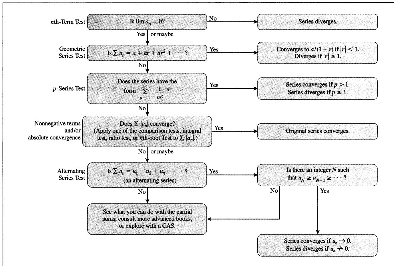
Flowchart 8.1 Procedure for Determining Convergence
