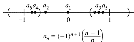
Neither the \epsilon -interval about 1 nor the \epsilon -interval about -1 contains a complete tail of the sequence.
