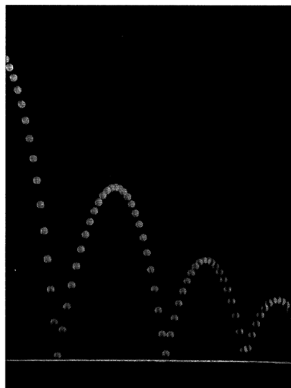
8.10 (a) Example 3 shows how to use a geometric series to calculate the total vertical distance traveled by a bouncing ball if the height of each rebound is reduced by the factor r . (b) A stroboscopic photo of a bouncing ball.
