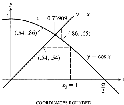
8.7 The solution of \cos x = x by Picard's method starting at x_0 = 1 (Example 9).
