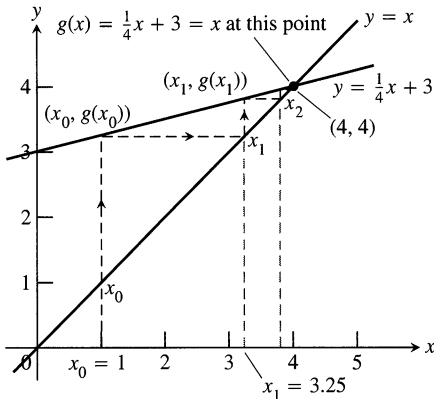
8.6 The Picard solution of the equation g(x) = (1/4)x + 3 = x (Example 8).
