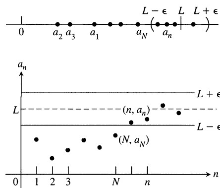
8.2 a_n \rightarrow L if y = L is a horizontal asymptote of the sequence of points \{(n, a_n)\} . In this figure, all the a_n 's after a_N lie within \epsilon of L .
