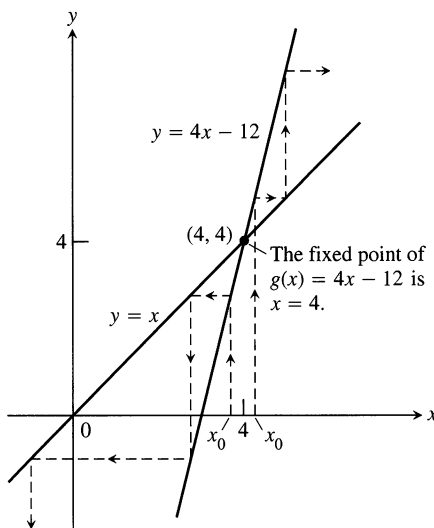
8.8 Applying the Picard method to g(x) = 4x - 12 will not find the fixed point unless x_0 is the fixed point 4 itself (Example 10).
