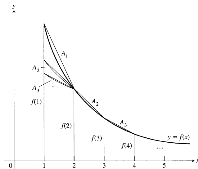
8.21 The figure for Exercise 19.
