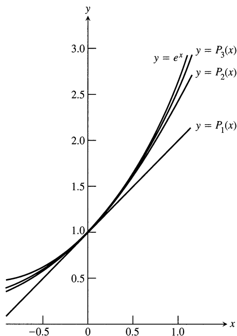
8.17 The graph of f(x) = e^x and its Taylor polynomials
