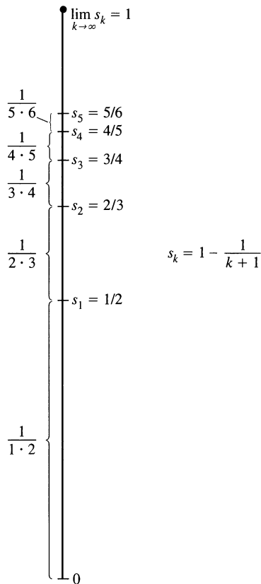
8.11 The partial sums of the series in Example 5.
