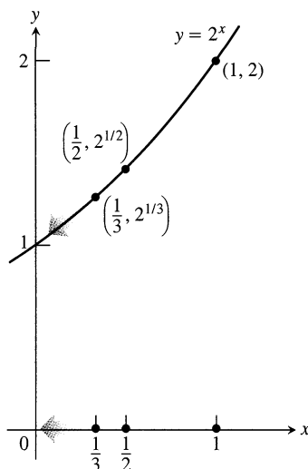
8.5 As n \rightarrow \infty , 1/n \rightarrow 0 and 2^{1/n} \rightarrow 2^0 .
