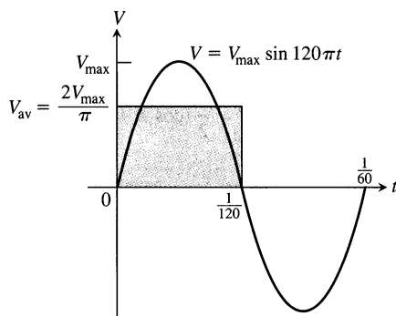
4.25 The graph of the household voltage V = V_{\max} \sin 120\pi t over a full cycle. Its average value over a half-cycle is 2V_{\max}/\pi . Its average value over a full cycle is zero.
