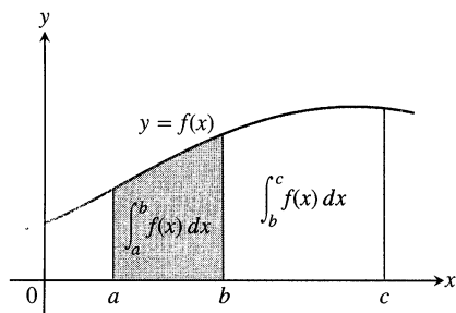
Figure 4.16 Additivity for definite integrals:
