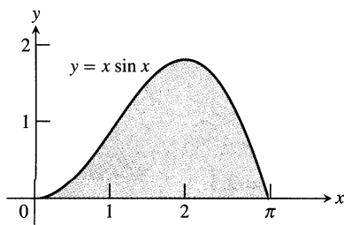
4.29 Graph of the integrand in Example 3.
