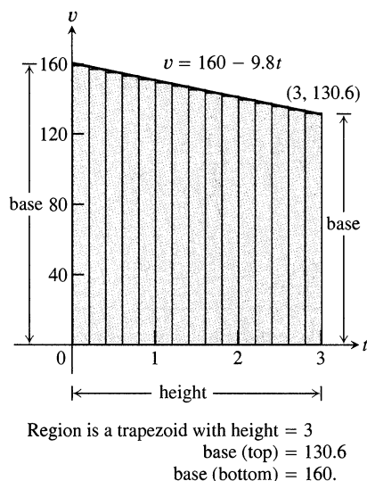
4.13 Rectangles for a Riemann sum of the velocity function f(t) = 160 - 9.8t over the interval [0, 3] .
