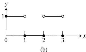
4.36 The graphs for Exercises 17 and 18.
