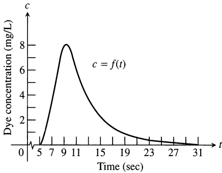
4.5 The dye concentrations from Table 4.3, plotted and fitted with a smooth curve. Time is measured with t = 0 at the time of injection. The dye concentrations are zero at the beginning, while the dye passes through the lungs. They then rise to a maximum at about t = 9 sec and taper to zero by t = 31 sec.
