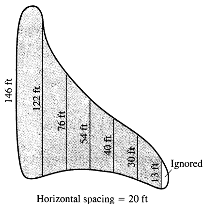
4.32 The swamp in Example 6.
