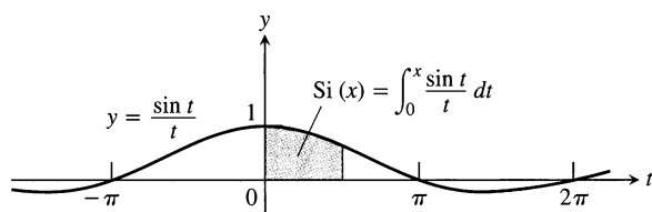
4.34 The continuous extension of y = (\sin t)/t . The sine-integral function \text{Si}(x) is the subject of Exercise 32.
