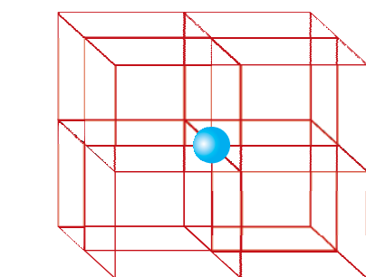
Fig. 1.12: In a simple cubic unit cell, each corner atom is shared between 8 unit cells.
