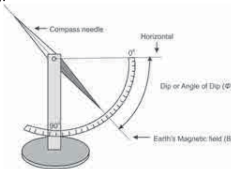
Fig. 12.7: Magnetic inclination.
