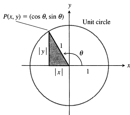
56 The acute reference triangle for an angle \theta .
