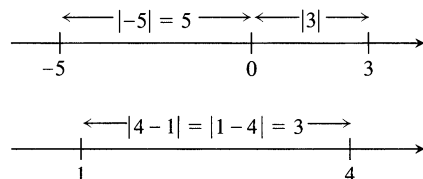
2 Absolute values give distances between points on the number line.
