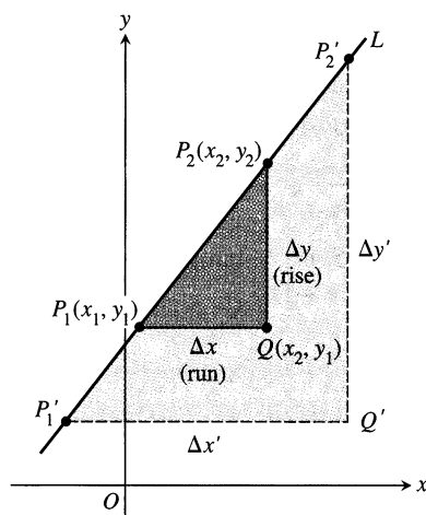
11 Triangles P_1QP_2 and P_1'Q'P_2' are similar, so
