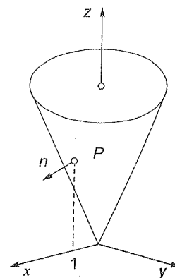
Cone and unit normal vector n
