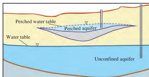
Fig. 6.4 : Perched Aquifer
