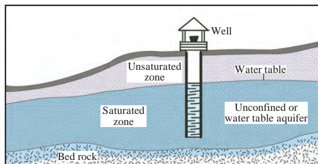
Fig. 6.3 : Unconfined Aquifer
