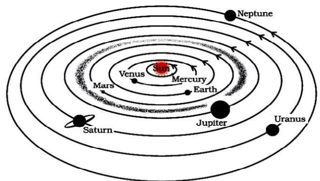
The solar system (not to scale)
