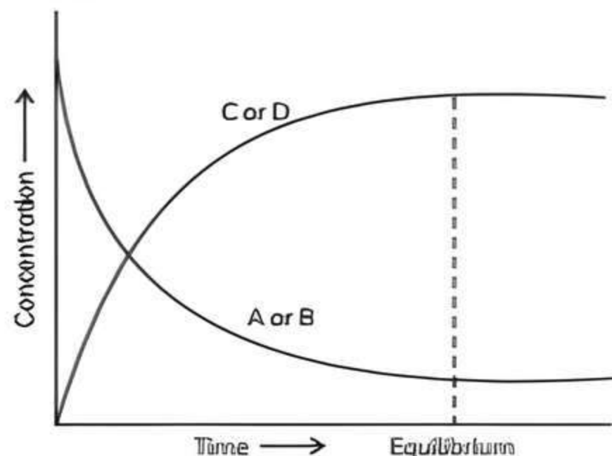
Attainment of chemical equilibrium.
