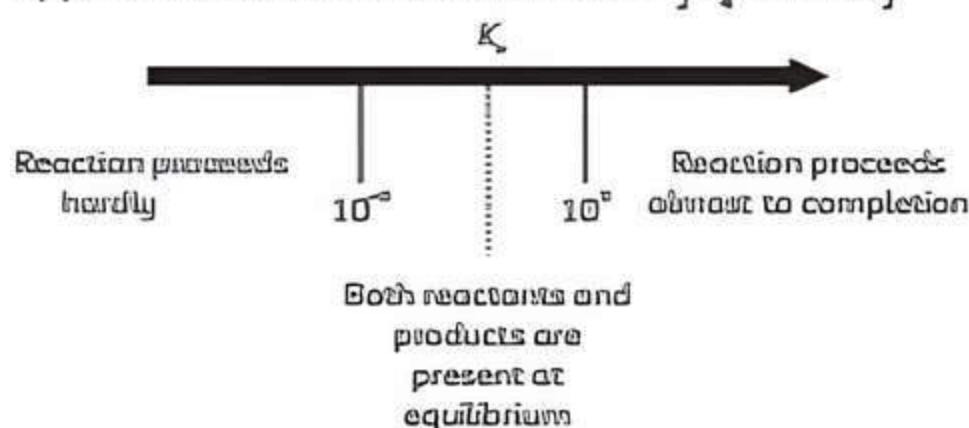
Predicting the extent of reaction based on K_c
