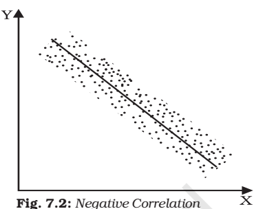
Fig. 7.2: Negative Correlation
