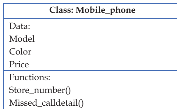
Fig 1: Class Mobile_phone
